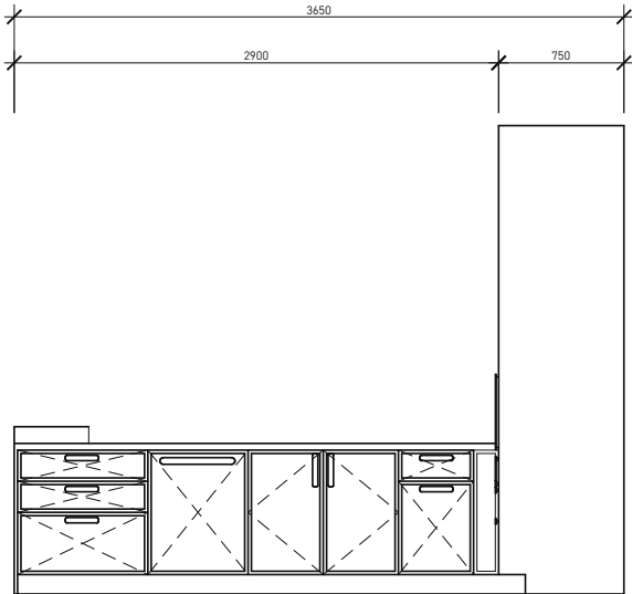
RIGHT SIDE ELEVATION SCALE 1:50
