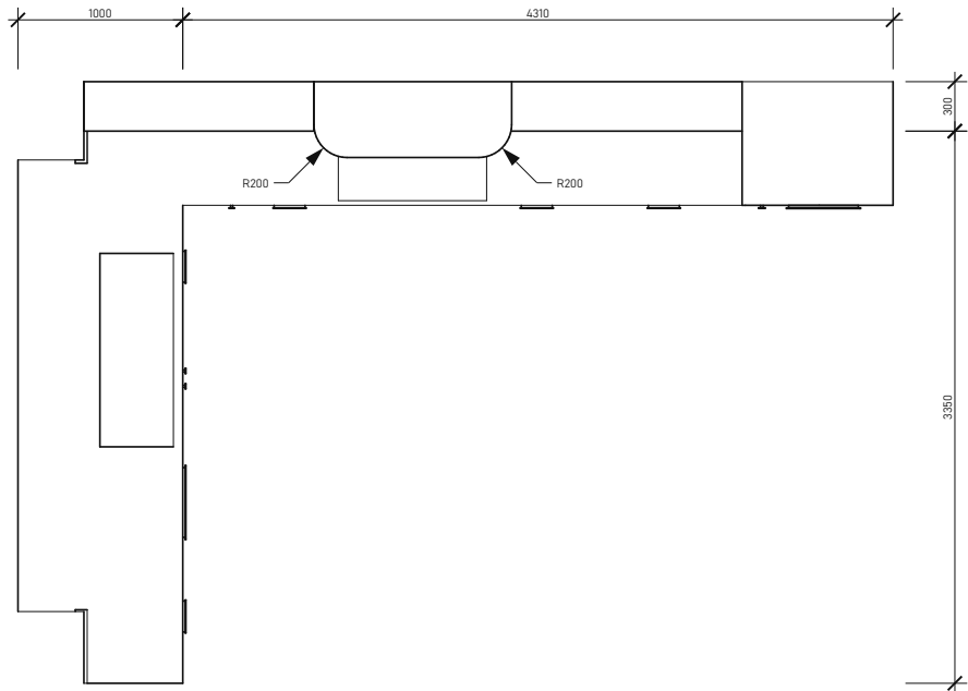
PLAN SCALE 1:50
